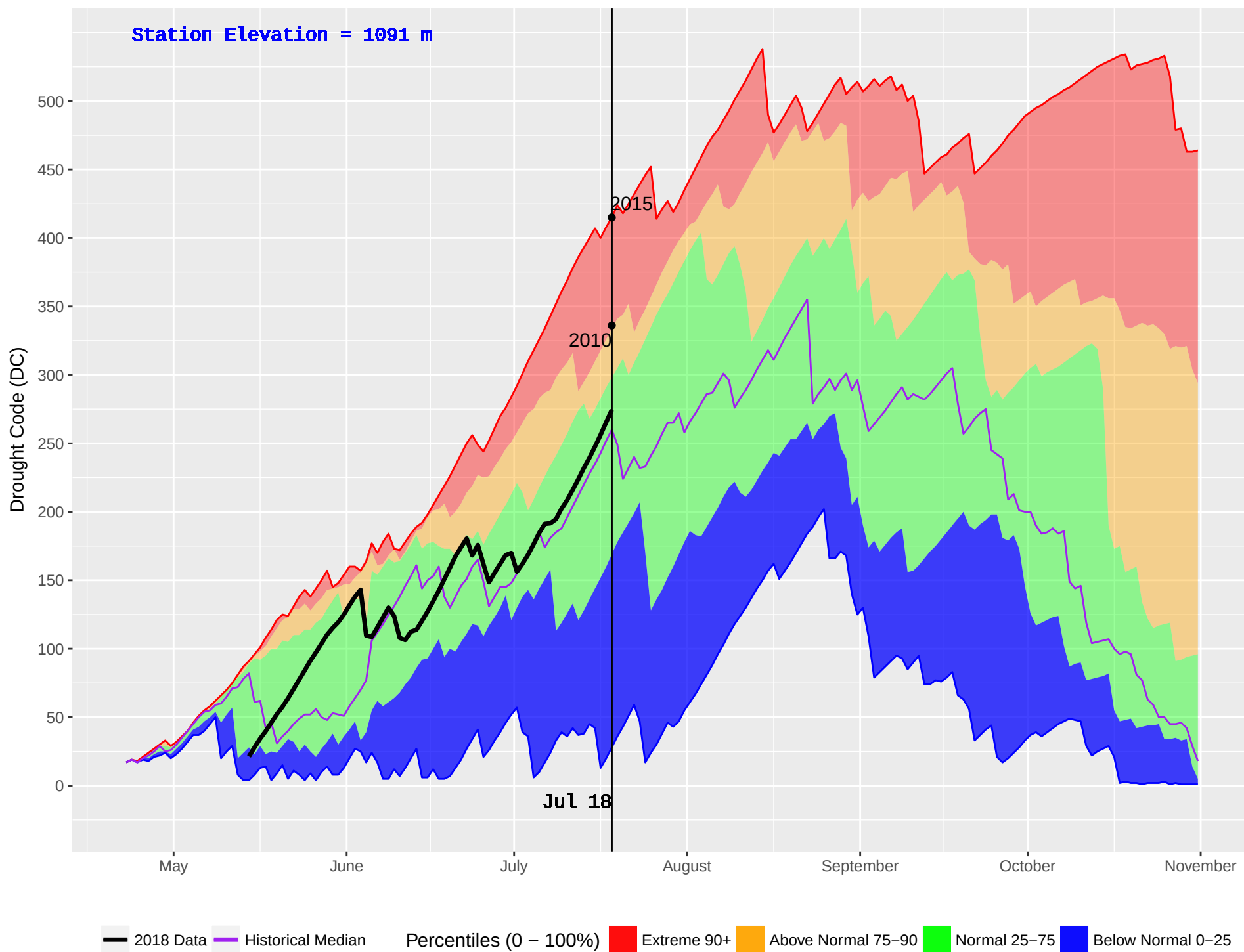
BIG MOUTH 2 (868) : Historical (2004–2016) and Current (2018) Daily Drought Code (DC)
